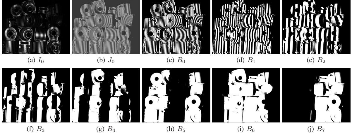
Figure 3: The principle of Time Multiplexed Binary Stripes when using a resolution of 8 bits.
