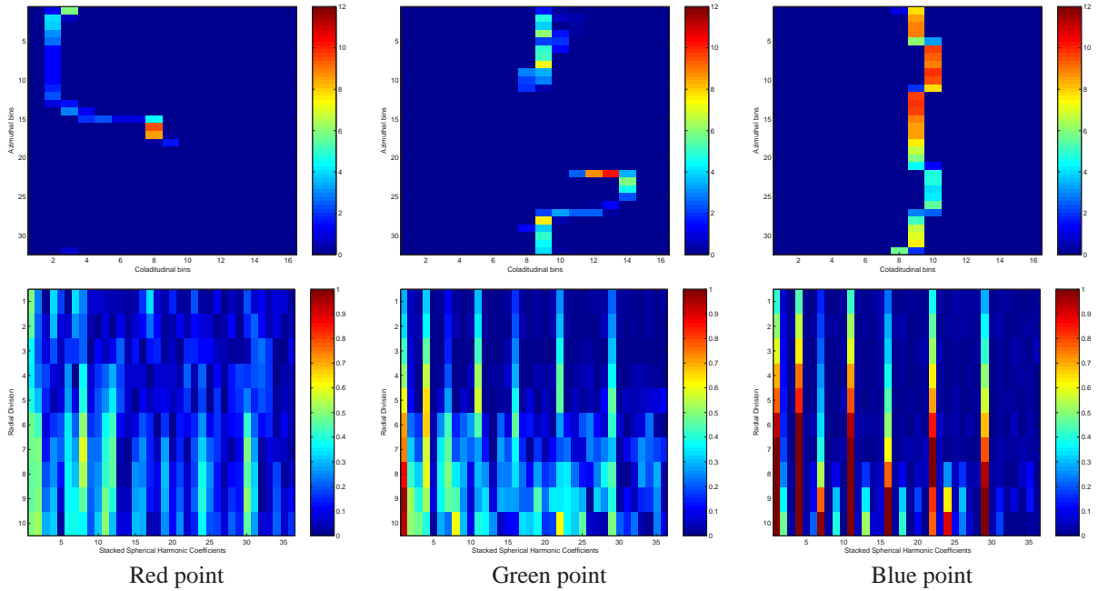
Figure 7: Illustrates shape contexts (first row) and harmonic shape contexts (second row) for the red, green, and blue points on the object mesh, respectively. Note that only the outer shell is visualized for the shape context and only the first 36 coefficients for the harmonic shape context.
