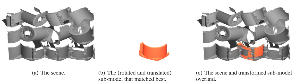
Figure 8: Depiction of a correct 5 degree of freedom pose estimation.
