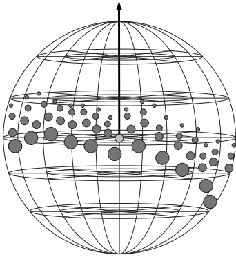
Figure 4: The spherical support region of the shape contexts.
