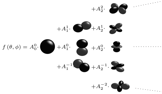
Figure 5: A spherical function expressed as a linear combination of spherical harmonic basis functions. Black indicates positive values and gray negative values.
